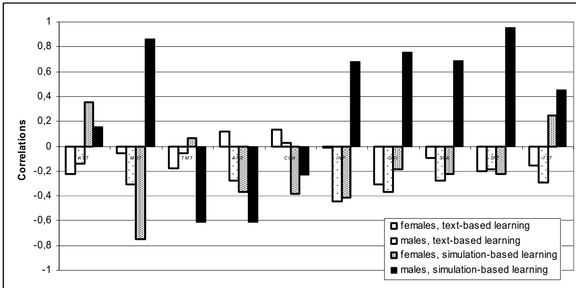
Figure 6: Correlations between LASSI subscale scores (ATT, MOT, TMT, ANX, CON, INP, SMI, STA, SFT, TST) and test performance for gender and type of learning object.
