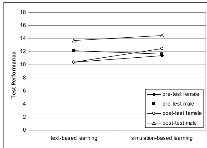
Figure 3: Performance in the post-test for gender and both learning groups.
