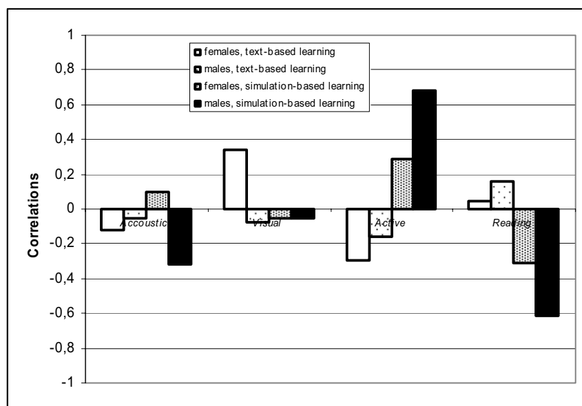
Figure 7: Correlations between HALB learning styles (acoustic, visual, active, reading) and test performance for gender and type of learning object.
