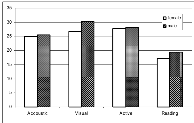
Figure 5: Scores in the HALB learning styles questionnaire for males and females.
