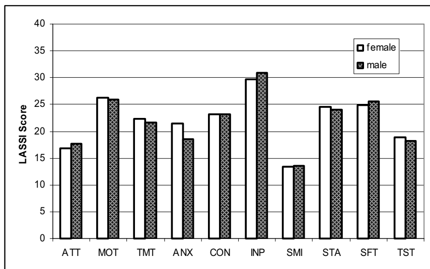
Figure 4: LASSI scores for males and females. The maximum score is 40, the minimum 0.
